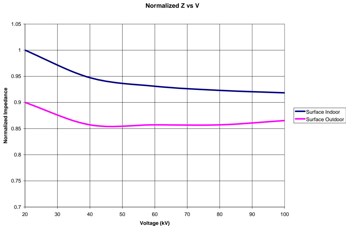
Figure 3. Plotted trends of Normalized Impedance vs. Applied Test Voltage
