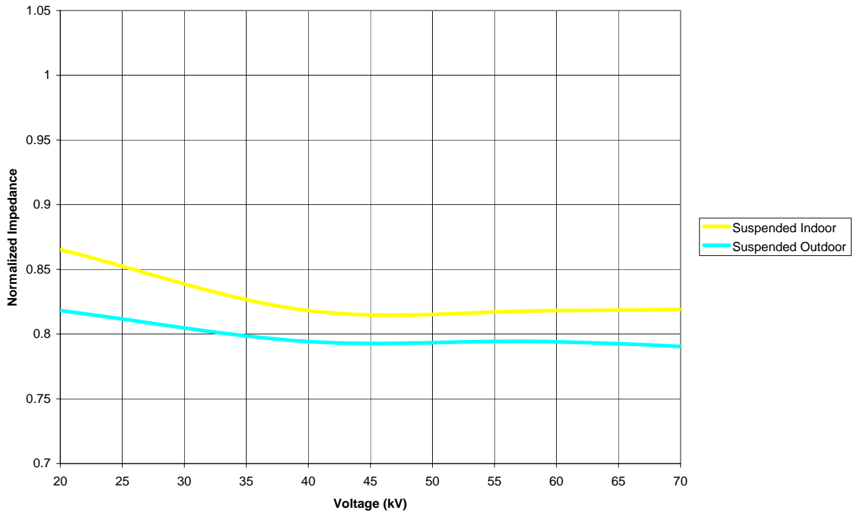
Figure 4. Effects of rerouting metering cables on impedance measurements
