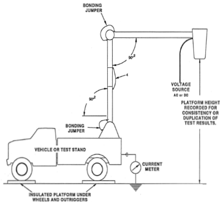
Figure 1. Dielectric Test Configuration for Category C Aerial Devices [1]
